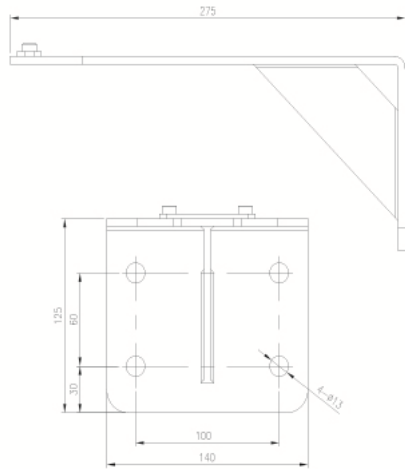
WALL BRACKET
