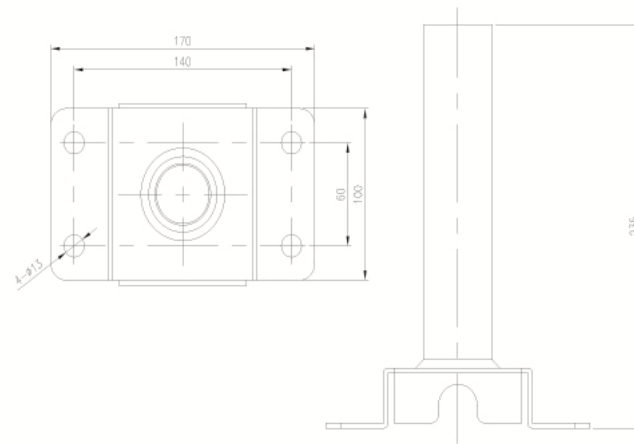
POLE BRACKET
